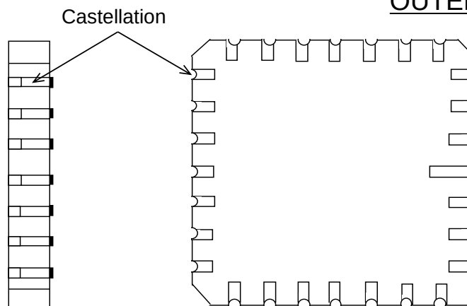
TYPE(1) (With Castellation)
